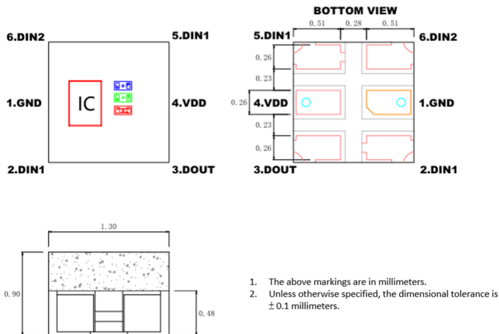
Figure 1. IN-PI13FTBT5R5G5B Package Outline Dimensions
