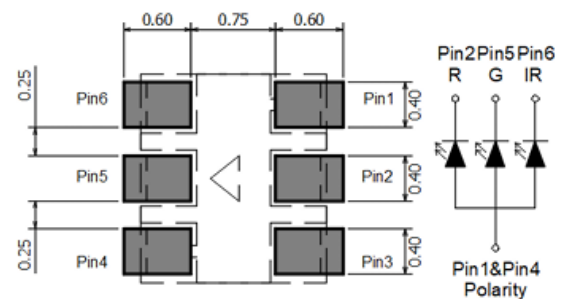
Figure 1. IN-S1816TATRGHIR Solder Pattern
