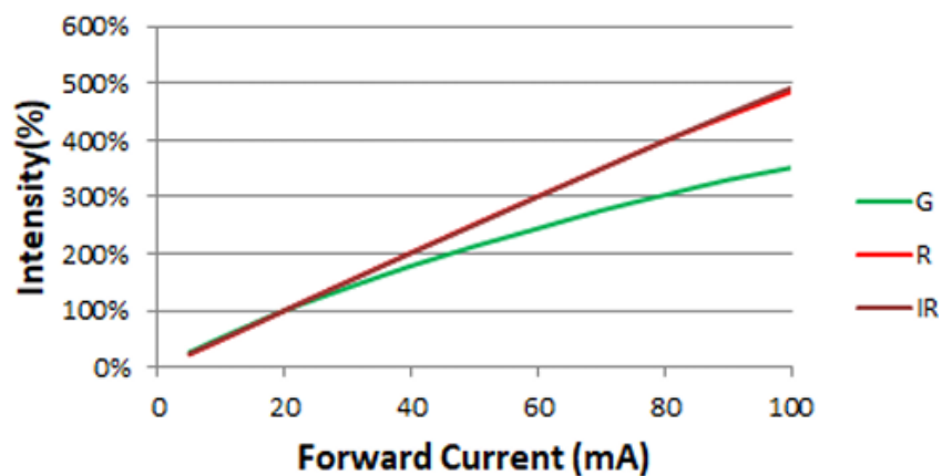
Relative Intensity vs. Forward Current
