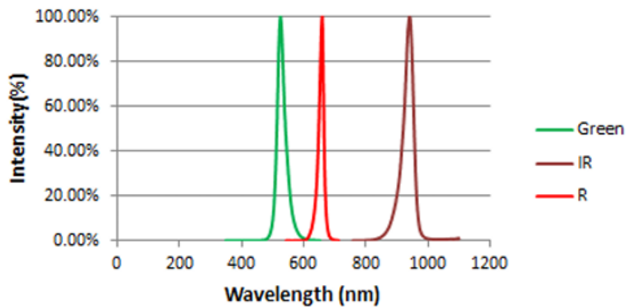
Relative Spectral Emission
