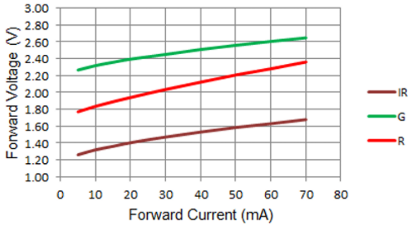
Forward Voltage VS. Forward Current
