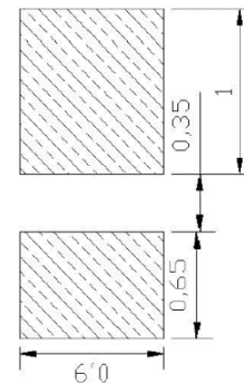
Figure 1. IN-P18ATA Solder Pattern
