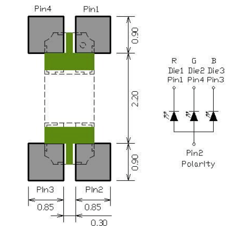
Figure 1. IN-S124TCR Solder Pattern
