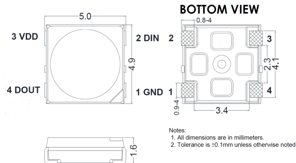
Figure 1. IN-PI55QATPRPGBPBW-XX Package Outline Dimensions
