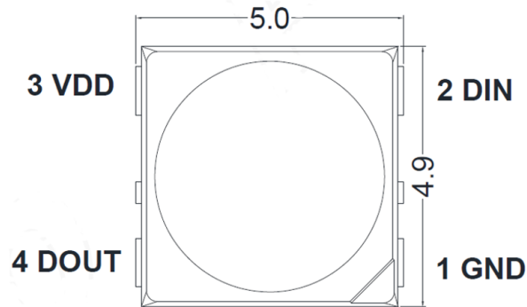
Figure 2. IN- PI55QATPRPGBPBW-XX Pin Configuration
