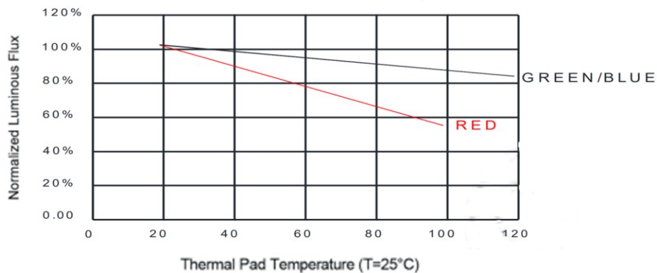
Thermal Pad Temperature vs. Relative Light Output
