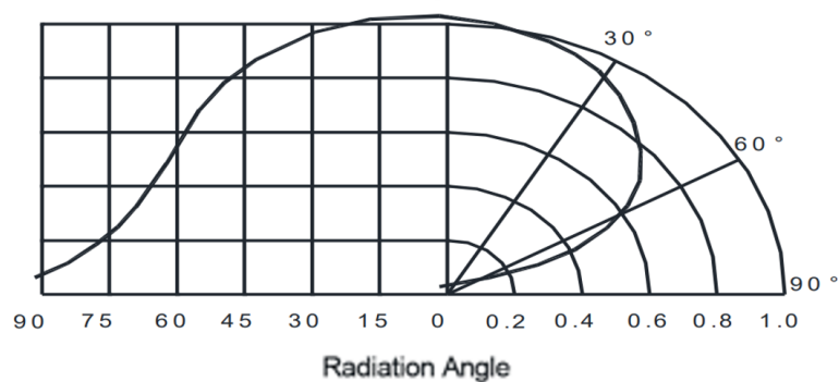
Typical Radiation Pattern 120°
