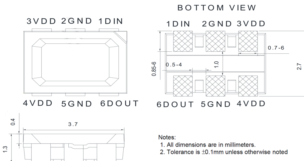
Figure 1. IN-PI3727TBTPRGPB Package Outline Dimensions
