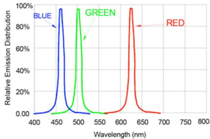
Wavelength Characteristics
