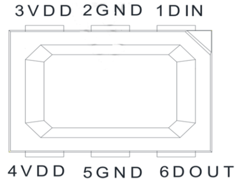
Figure 2. IN-PI3727TBTPRPGPB Pin Configuration
