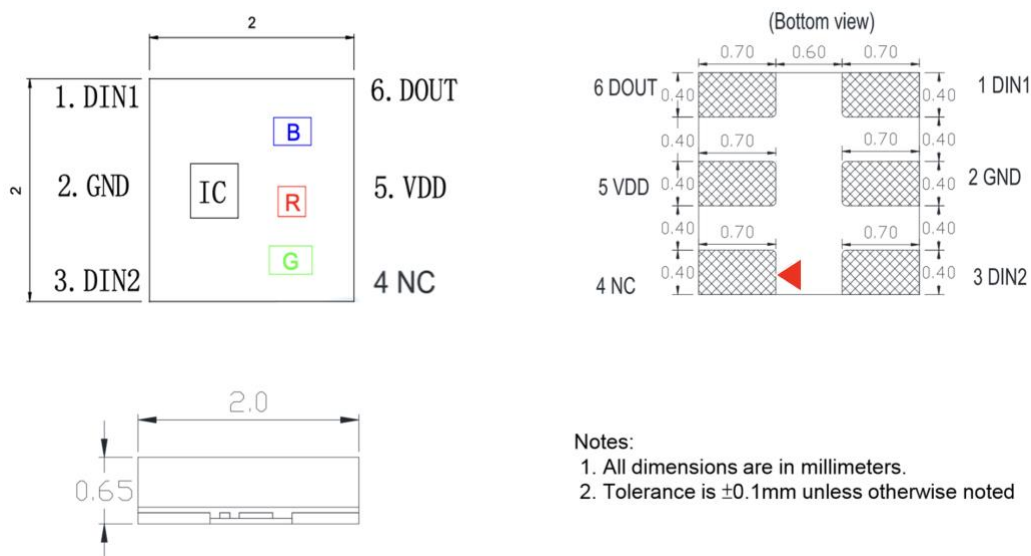
Figure 1. IN-PI20TBT5R5G5B Package Outline Dimensions
