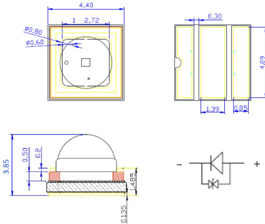
Figure 2. IN-C45PPATKU1 Package Dimension
