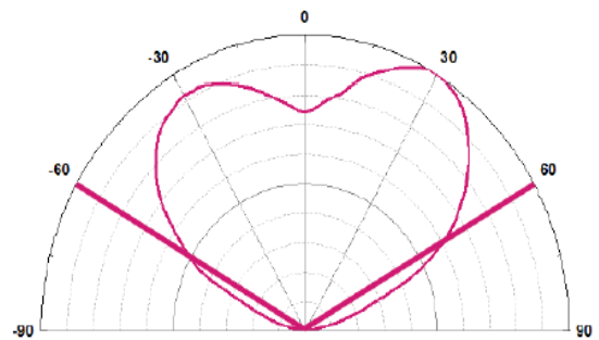
Radiation Characteristics
