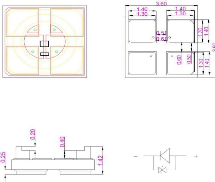
Figure 2. IN-C35PPCTGU1 Package Dimension
