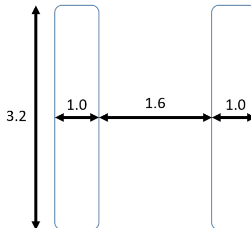
Figure 1. IN-C35PPCTGU1 Recommended Solder Pattern
