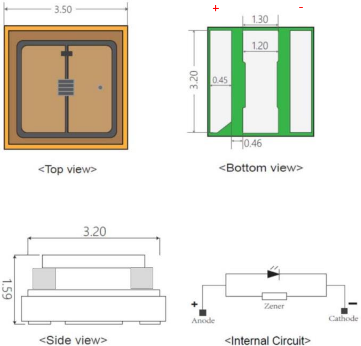
Figure 2. IN-C35PPCTLUB Package Dimension
