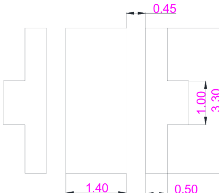
Figure 1. IN-C35PPCTLUB Recommended Solder Pattern
