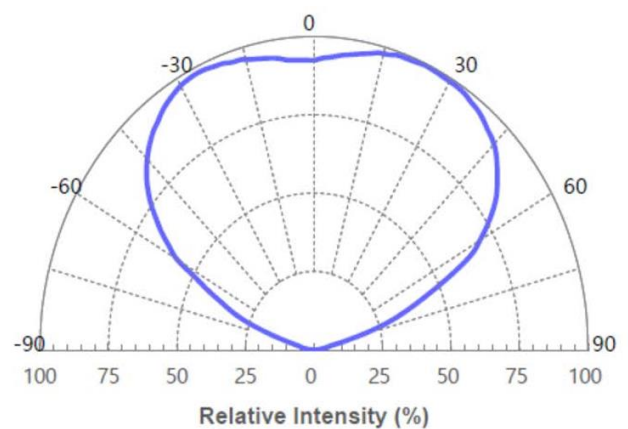
Radiation Characteristics
