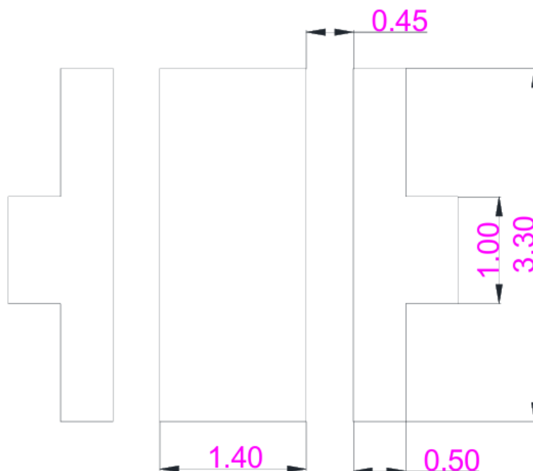
Figure 1. IN-C35PPCTGUB Recommended Solder Pattern
