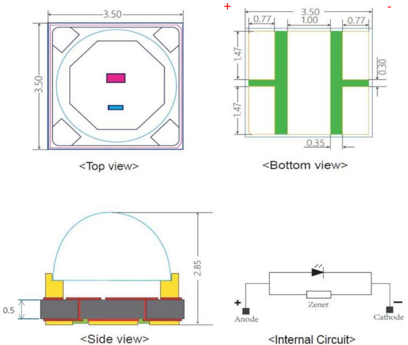
Figure 2. IN-C35PPBTLUB Package Dimension
