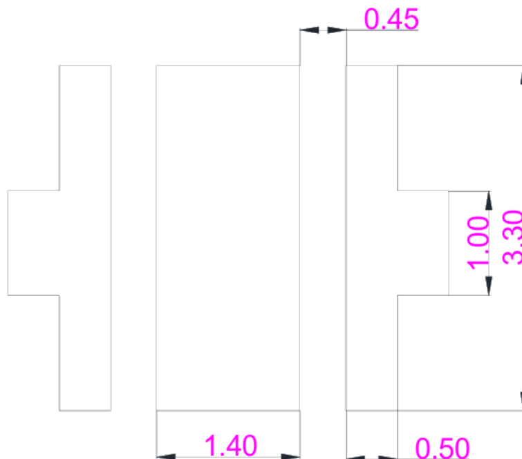
Figure 1. IN-C35PPBTLUB Recommended Solder Pattern
