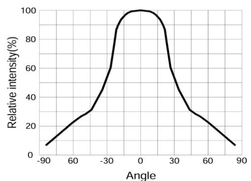
Radiation Characteristics
