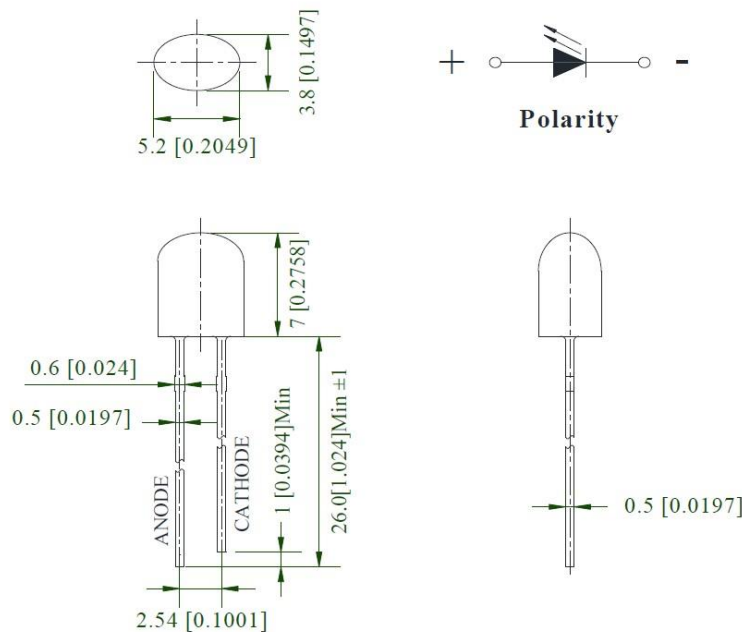
Figure 1. INO-5ABUB11040 Package Dimensions
