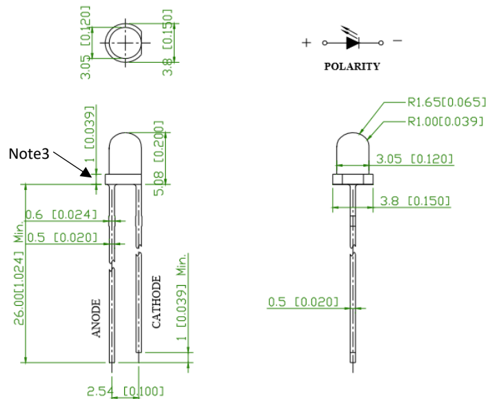
Figure 1. INL-3AX30 Package Dimensions
