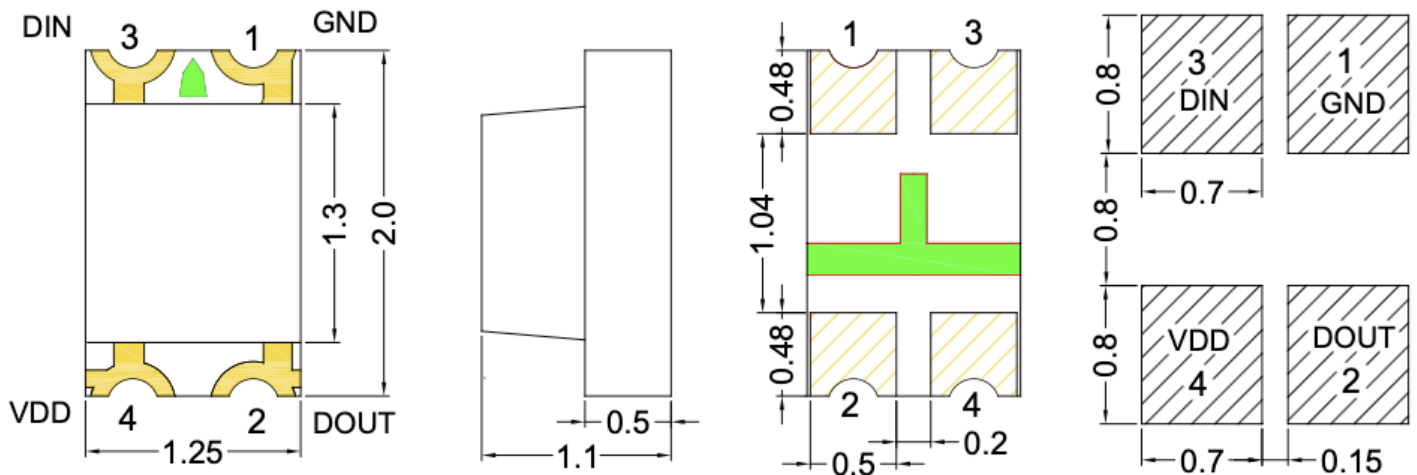
Figure 1. IN-PIS85ATPW Package Outline Dimensions
