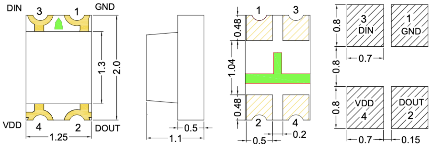
Figure 1. IN-PIS85ATPR Package Outline Dimensions
