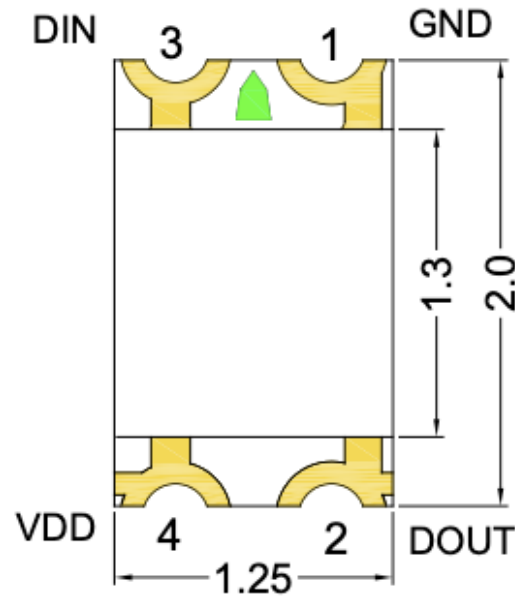
Figure 2. IN-PIS85ATPR Pin Configuration
