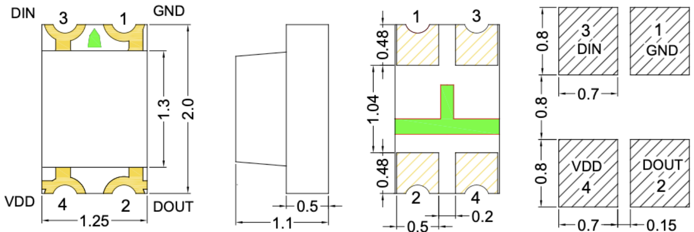
Figure 1. IN-PIS85ATPG Package Outline Dimensions
