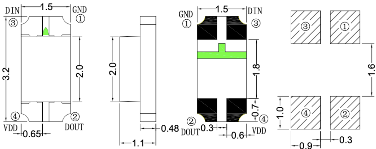
Figure 1. IN-PIS126ATPR Package Outline Dimensions
