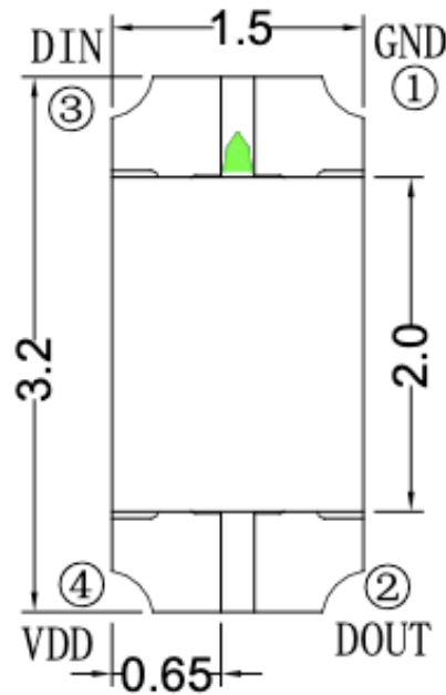
Figure 2. IN-PIS126ATPR Pin Configuration
