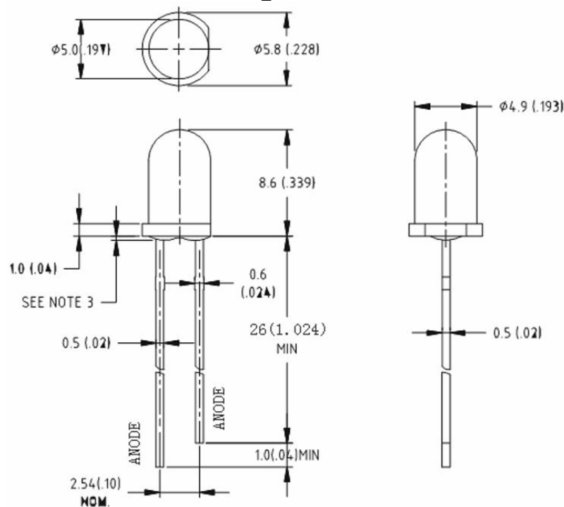
Figure 1. INL-5DB3UYYGP70 Package Dimensions
