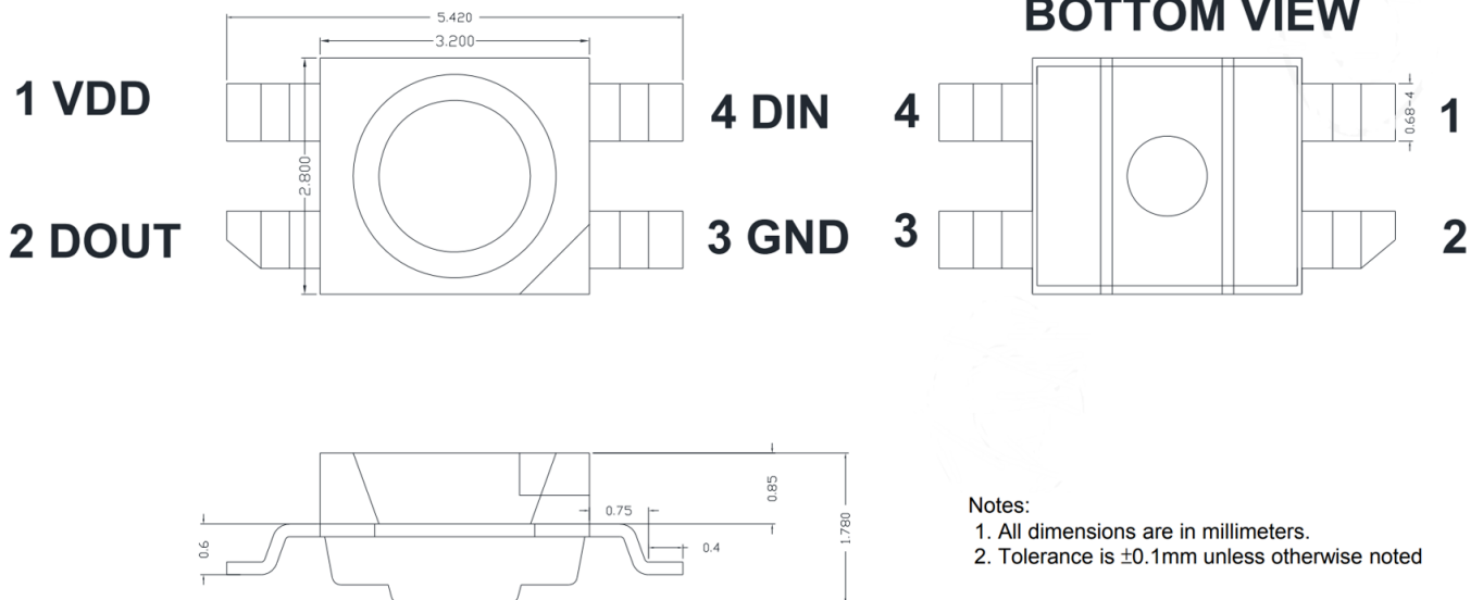
Figure 1. IN-PI32TATPRGPB.GR Package Outline Dimensions
