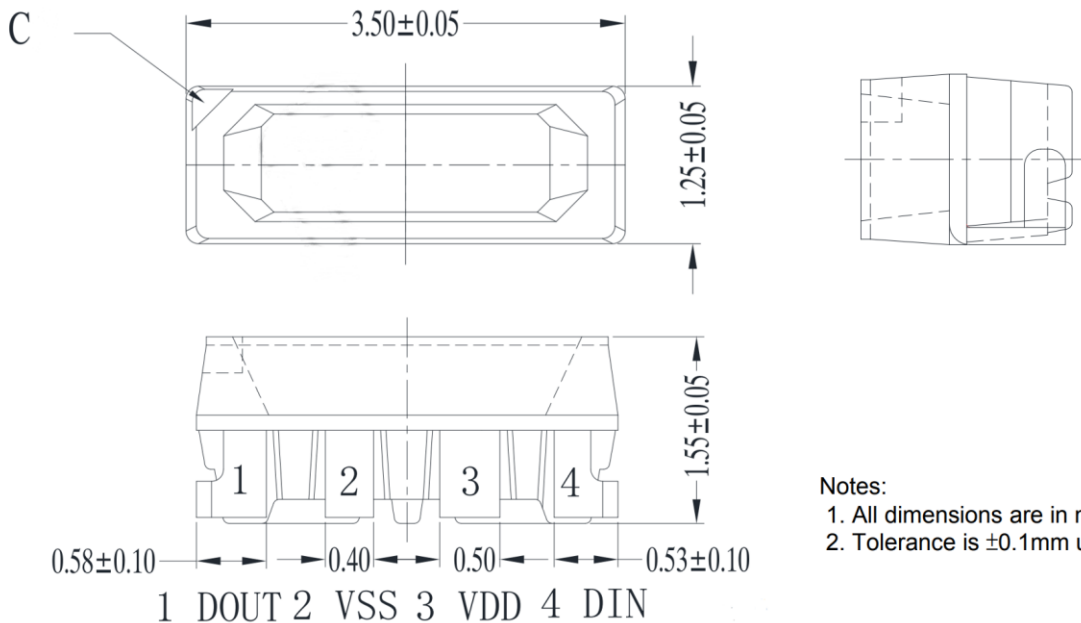
Figure 1. IN-PI31TAS5R5G5B Package Outline Dimensions
