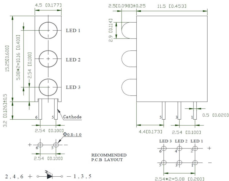
Figure 1. INH-3TXX80 series Package Dimensions
