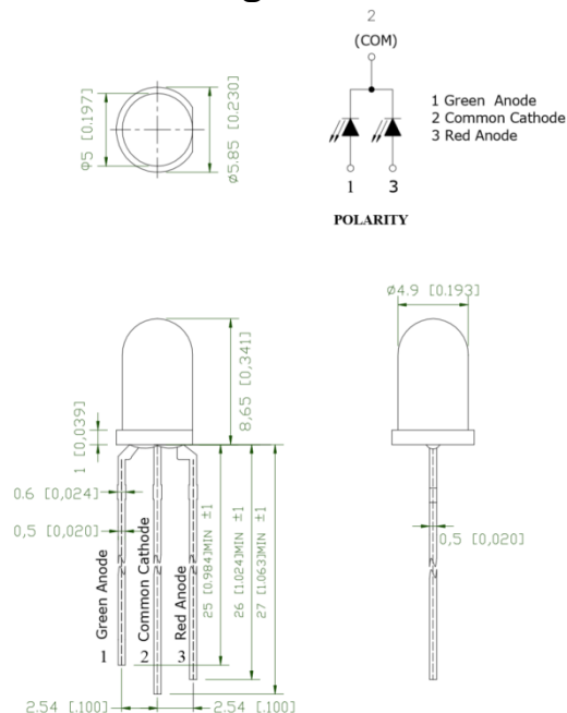
Figure 1. INL-5DB3URYGP60 Package Dimensions
