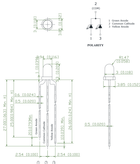
Figure 1. INL-3DA3UYYGP60 Package Dimensions
