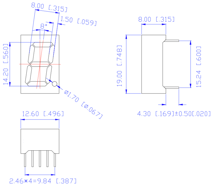
Figure 2. INND-TS56 series Package Dimensions
