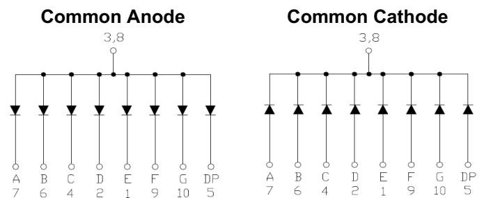
Figure 1. INND-SS56 series Internal Circuit Diagram
