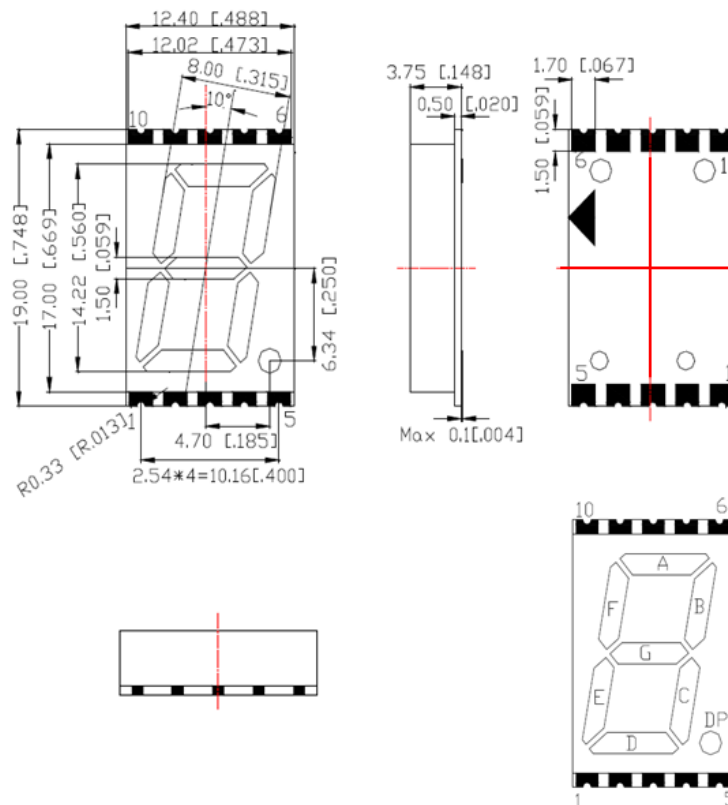
Figure 2. INND-SS56 series Package Dimensions
